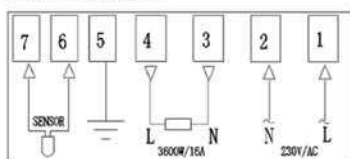
Water Heating System( Boiler)
