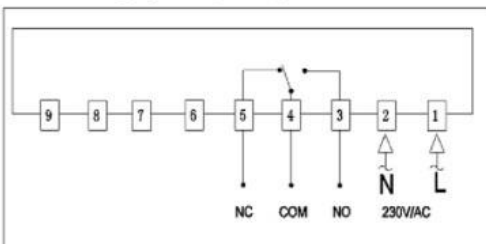
Voltage-Free System
