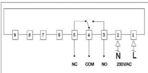
Voltage-Free System
