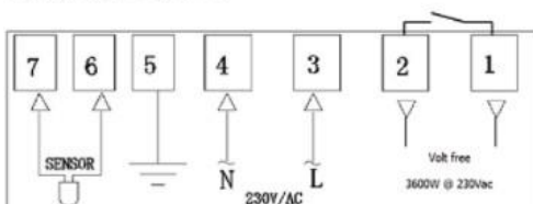
Voltage-Free System
